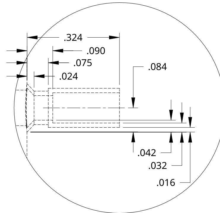
DETAIL A SCALE 5:1
